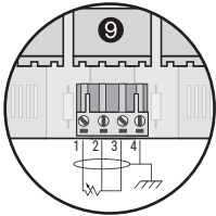
RTD connected directly to CRM board
